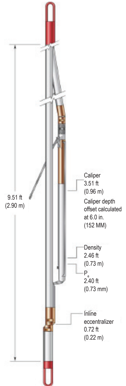
The Compact photodensity (MPD) tool can operate in memory or surface-readout mode.
