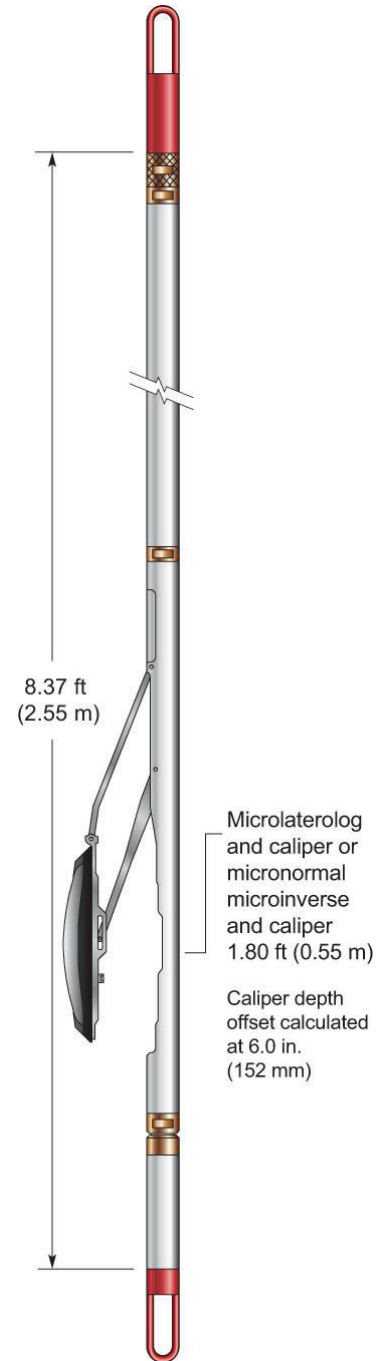
The Compact microresistivity (MMR/MML) tool provides resistivity measurements with memory or surface readout capability.
